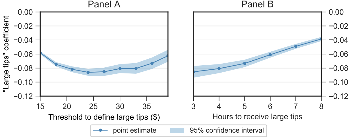
Figure 2: Coefficient's sensitivity to different thresholds
